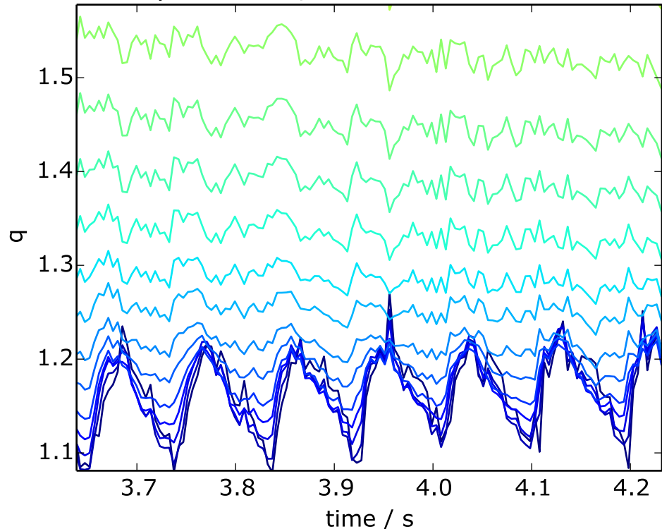
q evolution, rho=0.06:0.04:0.50
