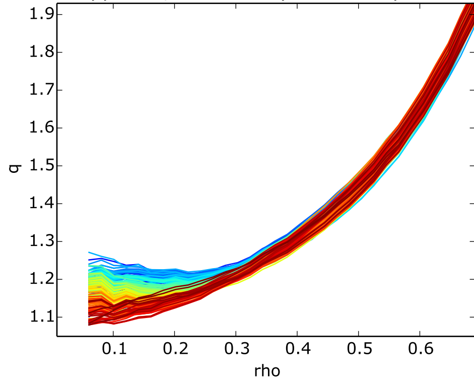
q profile, coloured by sawtooth phase
