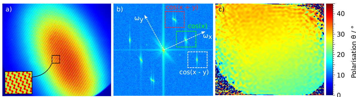
Figure 2: a) Typical IMSE image (zoomed area shows fringes), b) Fourier transform and c) demodulated polarisation map \theta(x,y)
