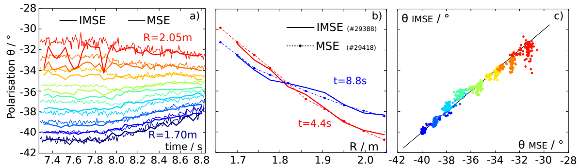
Figure 4: Comparison of MSE data and average of equivalent IMSE image region during a near identical plasma shot: a) Time traces during plasma current ramp down, b) Profiles during flat top (4.4s) and at end of ramp down (8.8s), c) Correlation over full shot. An unexplained 1.0^\circ offset is removed from the IMSE data.
