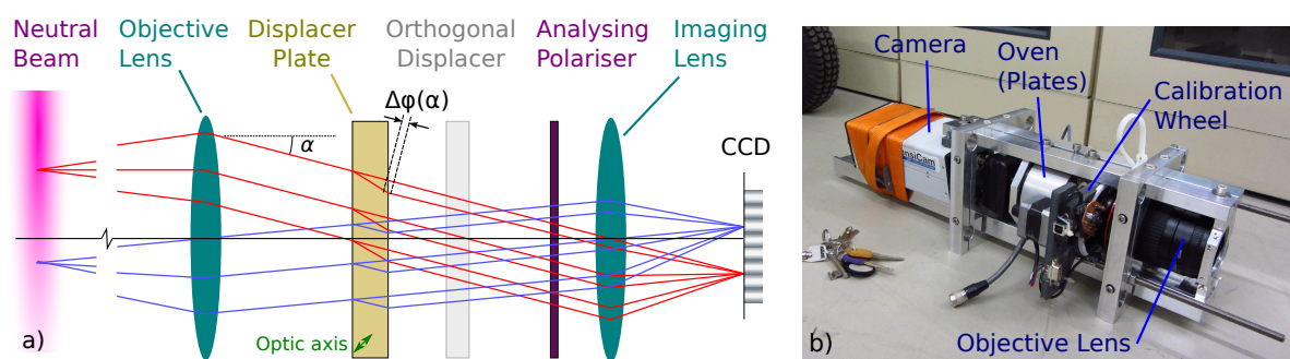
Figure 1: a) Basic IMSE system: Two lenses form an image of the beam emission on a CCD. A birefringent crystal with 45° tilted optic axis (Displacer) delays one polarisation by an angle dependant phase \Delta\phi(\alpha) and with an analysing polariser creates an interference pattern across the image. A second displacer creates an orthogonal pattern and the ratio of their amplitudes relates to the input polarisation angle. b) Photograph of the compact prototype ASDEX Upgrade IMSE diagnostic.
