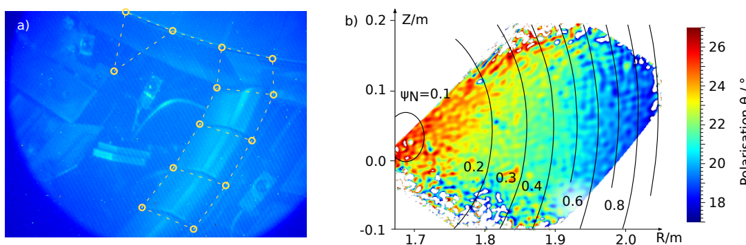
Figure 3: a) Background image (no beams) with identified known points. b) Transformed polarisation image in (R,Z) at beam intersection plane (source 3 in this case).
