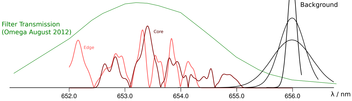
Spectrum for April 22nd 2013 (Hydrogen Beams)
