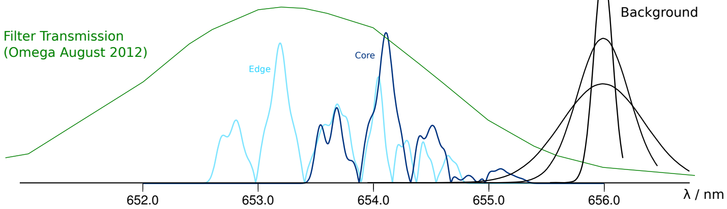
Spectrum for January 2013 (Deuterium Beams)
