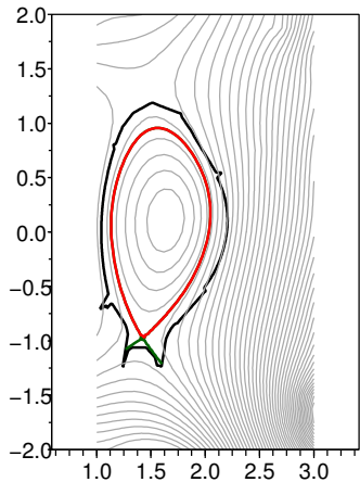
psi, LCFS and firstwall
