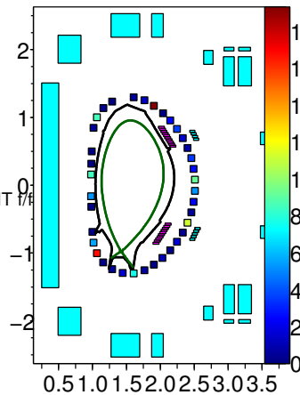
Sensors chi^2
