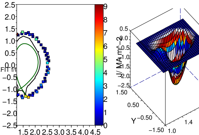
Sensors chi^2
