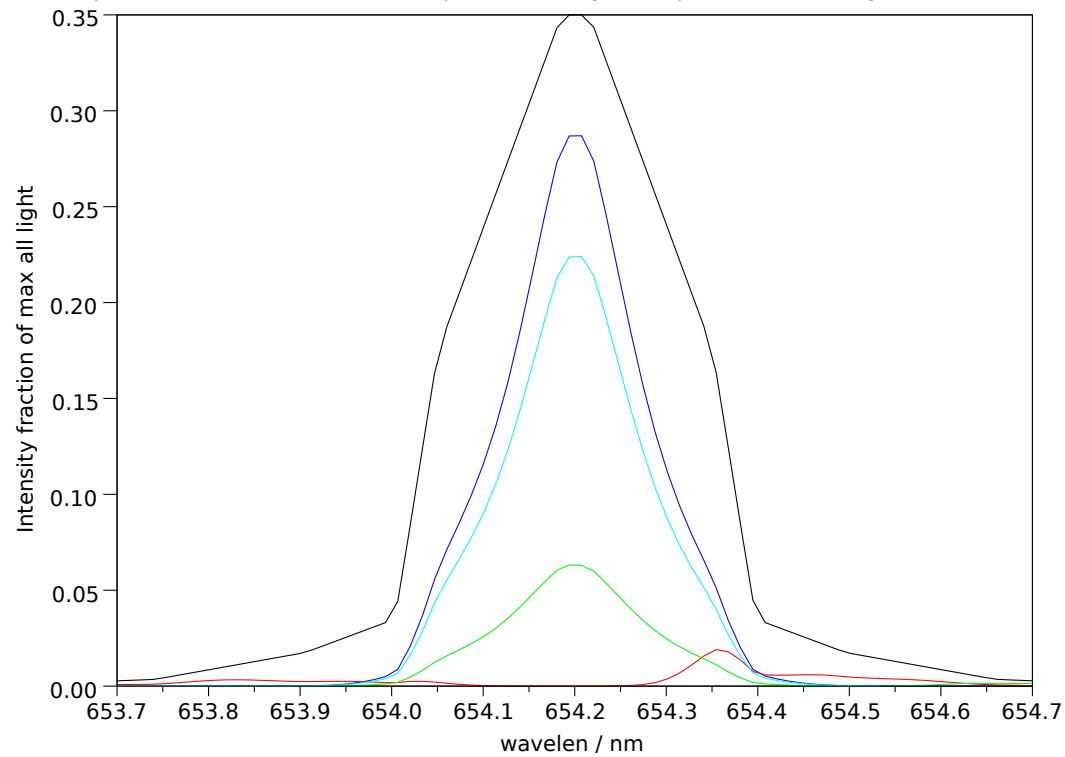
Filter 2: Makeup: Good= 78.0%, bad= 4.6%, unpol= 17.4% , good-unpol=60.6%. Total good transmitted= 24.8%
