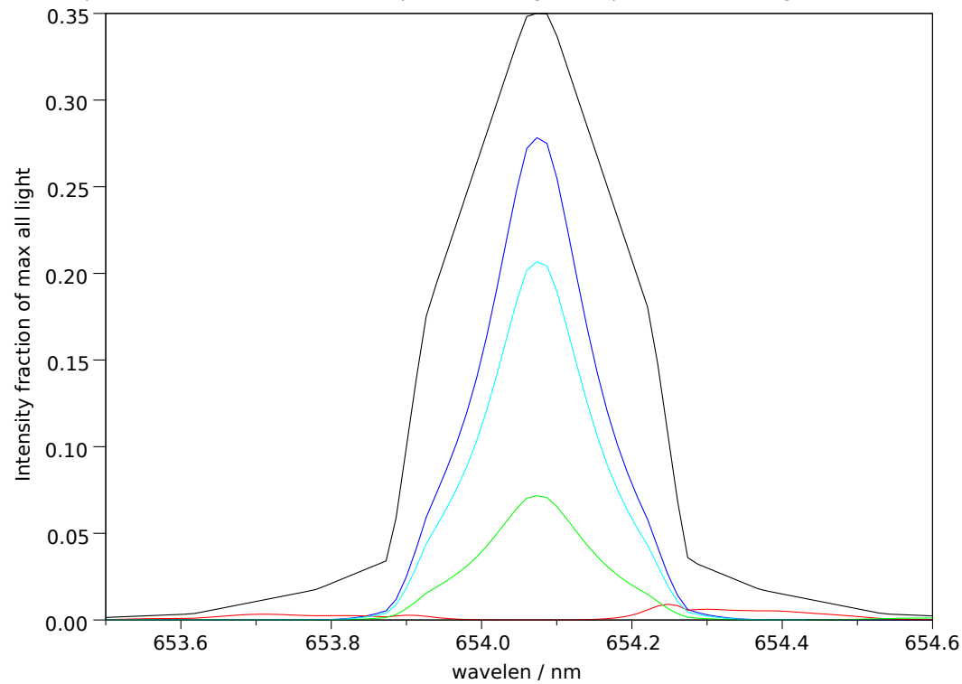
Filter 2: Makeup: Good= 76.5%, bad= 3.7%, unpol= 19.7% , good-unpol=56.8%. Total good transmitted= 25.0%
