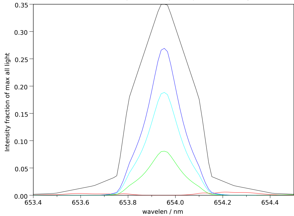
Filter 2: Makeup: Good= 74.5%, bad= 3.4%, unpol= 22.2% , good-unpol=52.3%. Total good transmitted= 25.2%
