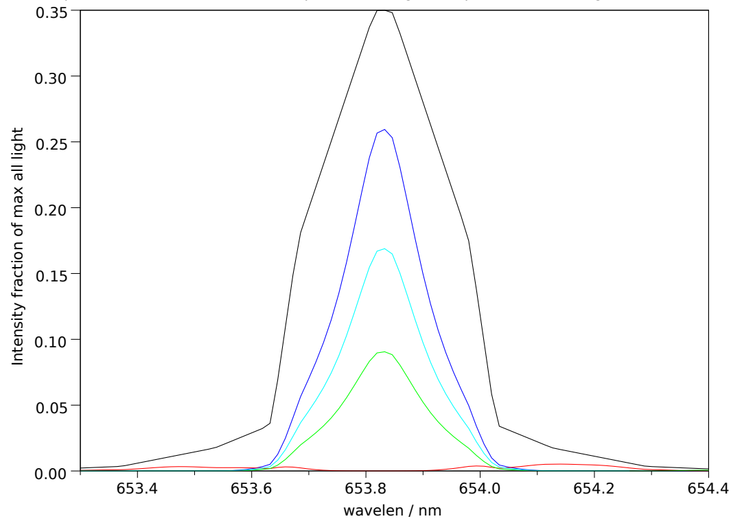
Filter 2: Makeup: Good= 72.1%, bad= 3.2%, unpol= 24.7% , good-unpol=47.3%. Total good transmitted= 25.3%
