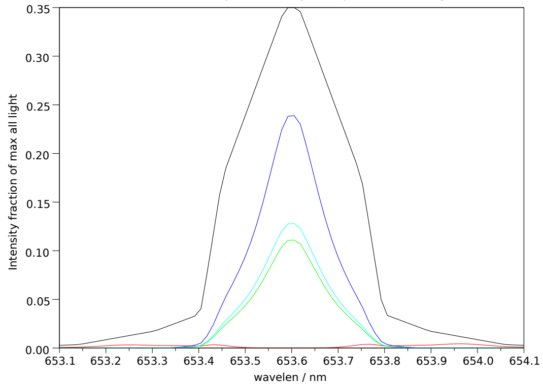
Filter 2: Makeup: Good= 66.9%, bad= 2.8%, unpol= 30.3% , good-unpol=36.7%. Total good transmitted= 25.6%
