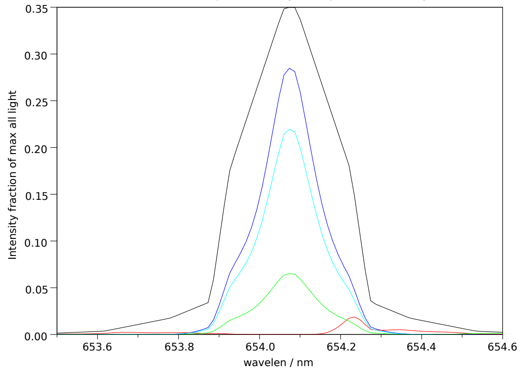
Filter 2: Makeup: Good= 78.1%, bad= 3.9%, unpol= 18.0% , good-unpol=60.1%. Total good transmitted= 23.9%
