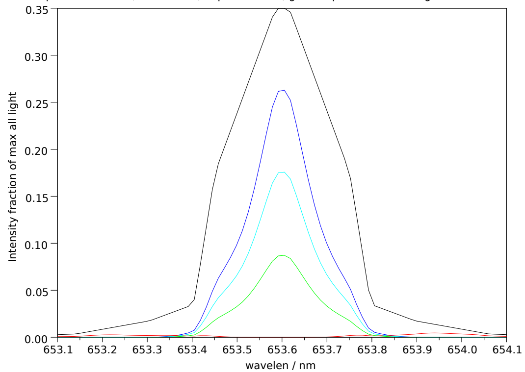
Filter 2: Makeup: Good= 74.1%, bad= 2.3%, unpol= 23.6% , good-unpol=50.5%. Total good transmitted= 24.6%
