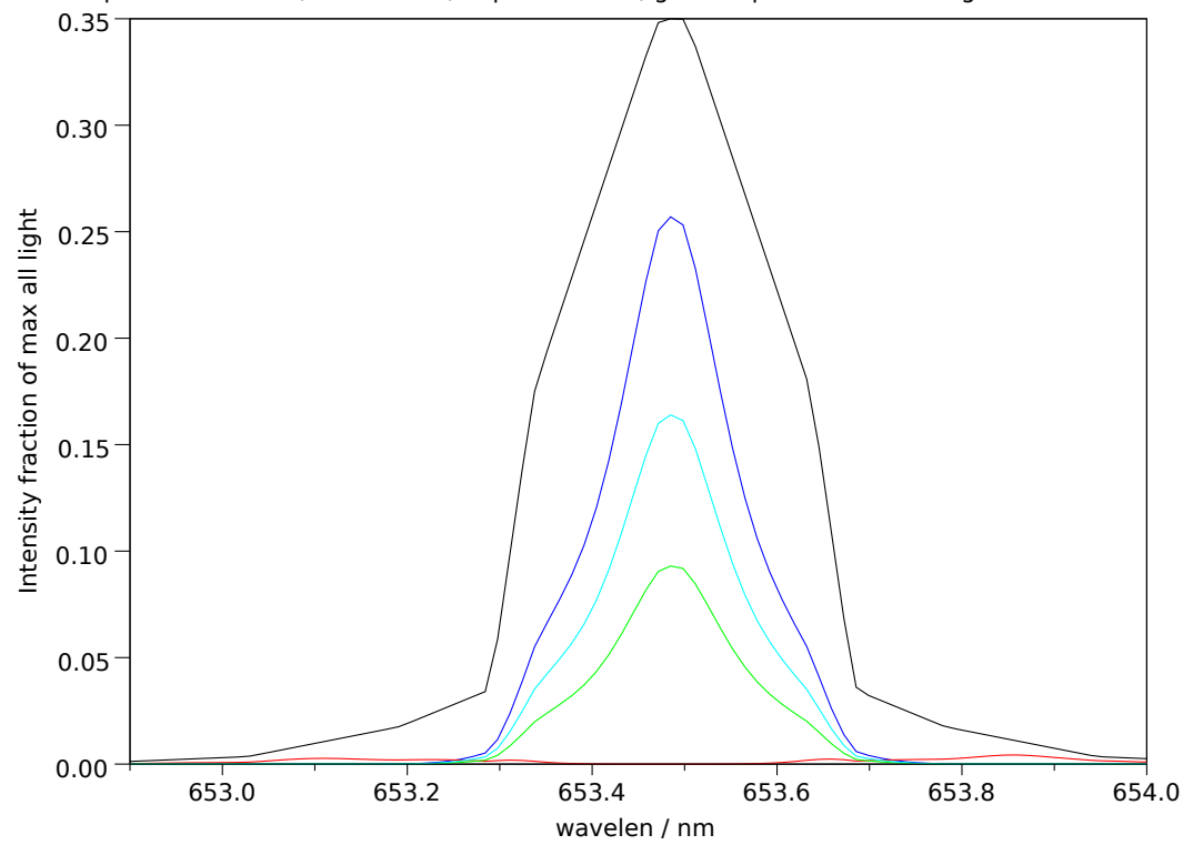
Filter 2: Makeup: Good= 72.8%, bad= 2.1%, unpol= 25.1% , good-unpol=47.6%. Total good transmitted= 24.8%
