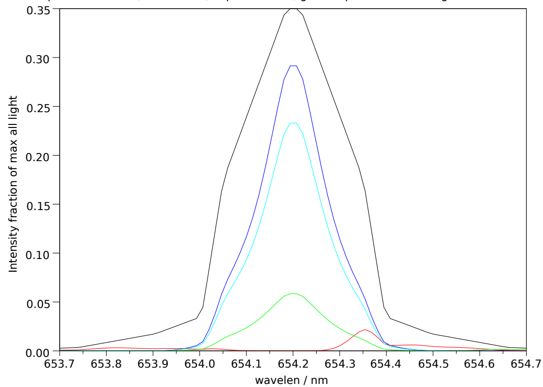
Filter 2: Makeup: Good= 79.1%, bad= 4.8%, unpol= 16.2% , good-unpol=62.9%. Total good transmitted= 24.6%
