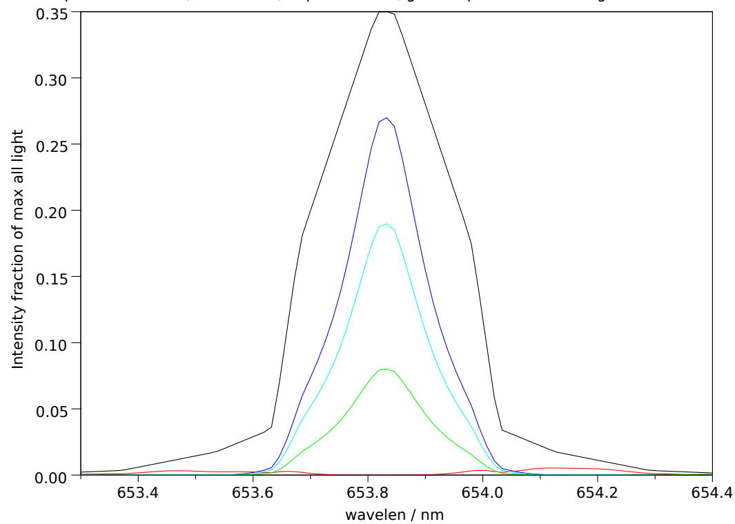
Filter 2: Makeup: Good= 75.0%, bad= 3.2%, unpol= 21.8% , good-unpol=53.2%. Total good transmitted= 25.1%
