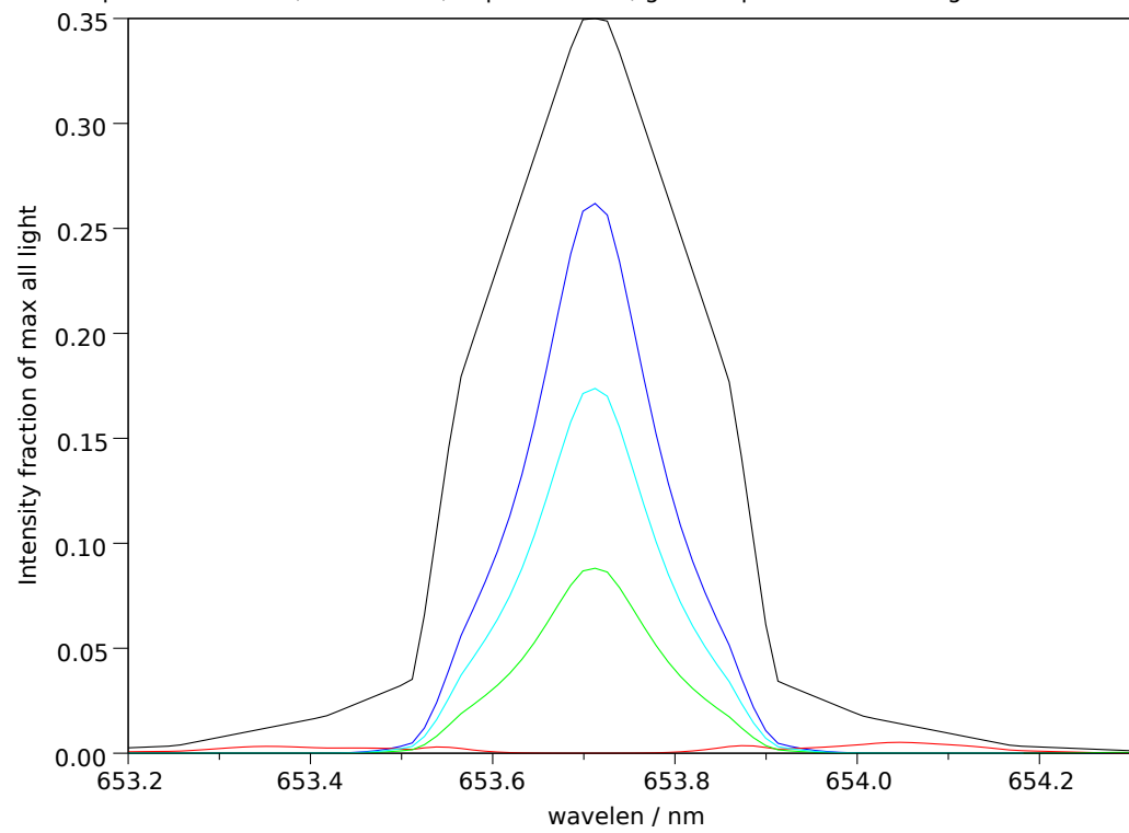
Filter 2: Makeup: Good= 73.1%, bad= 3.0%, unpol= 23.9% , good-unpol=49.2%. Total good transmitted= 25.3%
