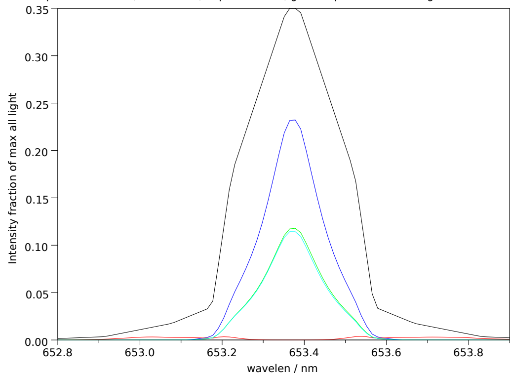
Filter 2: Makeup: Good= 65.7%, bad= 2.2%, unpol= 32.1% , good-unpol=33.7%. Total good transmitted= 25.7%
