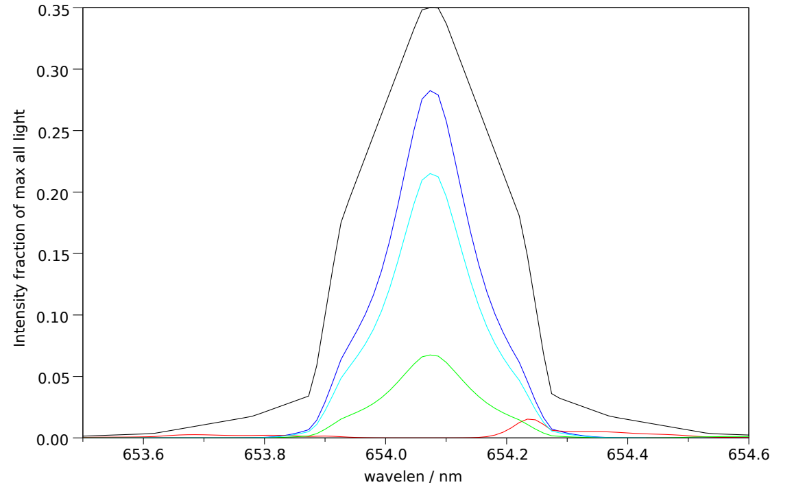
Filter 2: Makeup: Good= 77.6%, bad= 3.8%, unpol= 18.6% , good-unpol=59.0%. Total good transmitted= 24.3%
