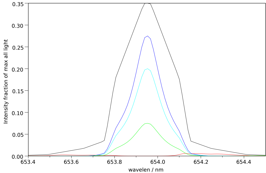
Filter 2: Makeup: Good= 76.4%, bad= 3.0%, unpol= 20.7% , good-unpol=55.7%. Total good transmitted= 24.5%
