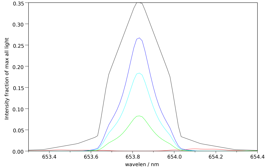
Filter 2: Makeup: Good= 74.5%, bad= 2.7%, unpol= 22.8% , good-unpol=51.8%. Total good transmitted= 24.6%
