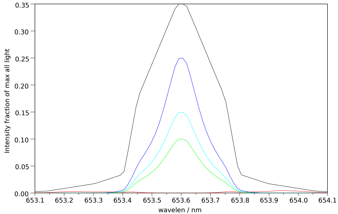
Filter 2: Makeup: Good= 70.4%, bad= 2.4%, unpol= 27.3% , good-unpol=43.1%. Total good transmitted= 24.9%
