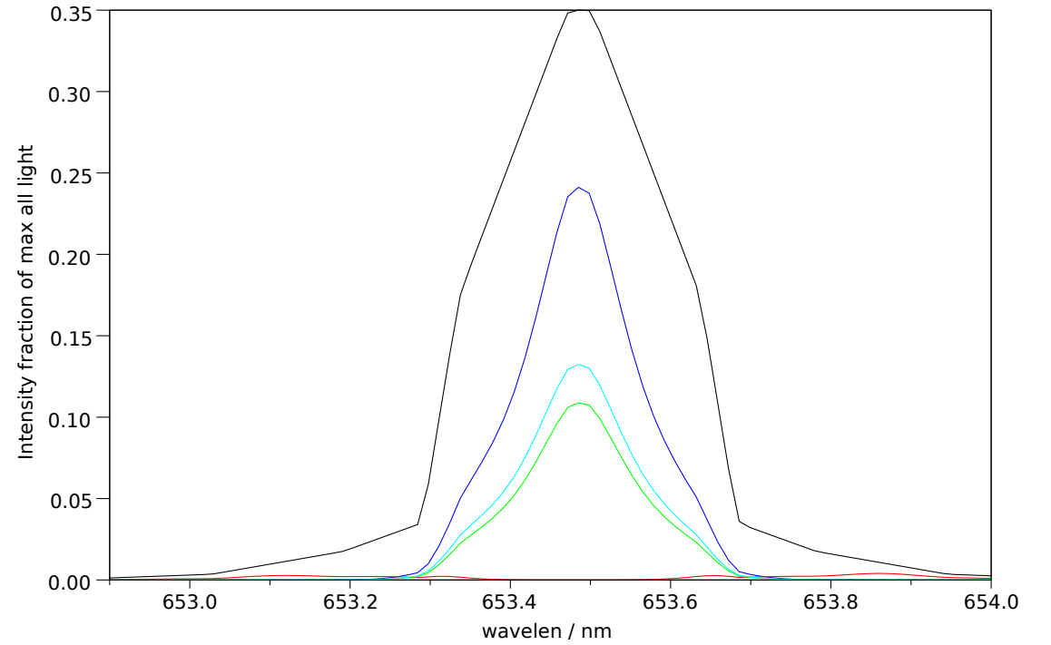
Filter 2: Makeup: Good= 68.2%, bad= 2.1%, unpol= 29.6% , good-unpol=38.6%. Total good transmitted= 25.1%
