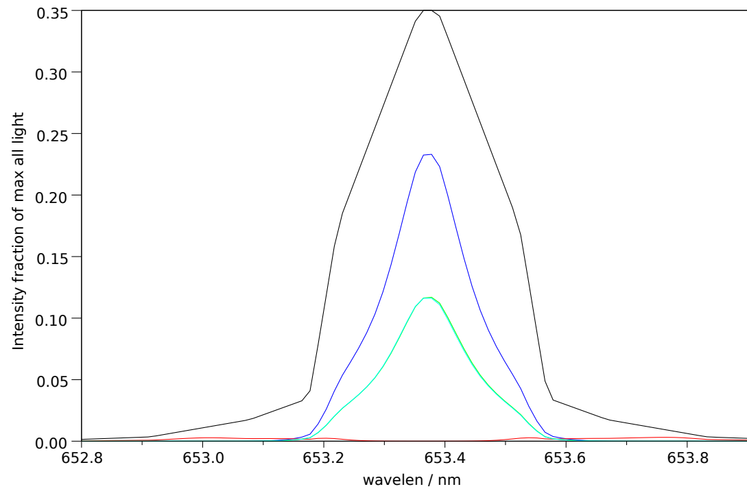
Filter 2: Makeup: Good= 66.3%, bad= 1.8%, unpol= 31.9% , good-unpol=34.5%. Total good transmitted= 25.2%
