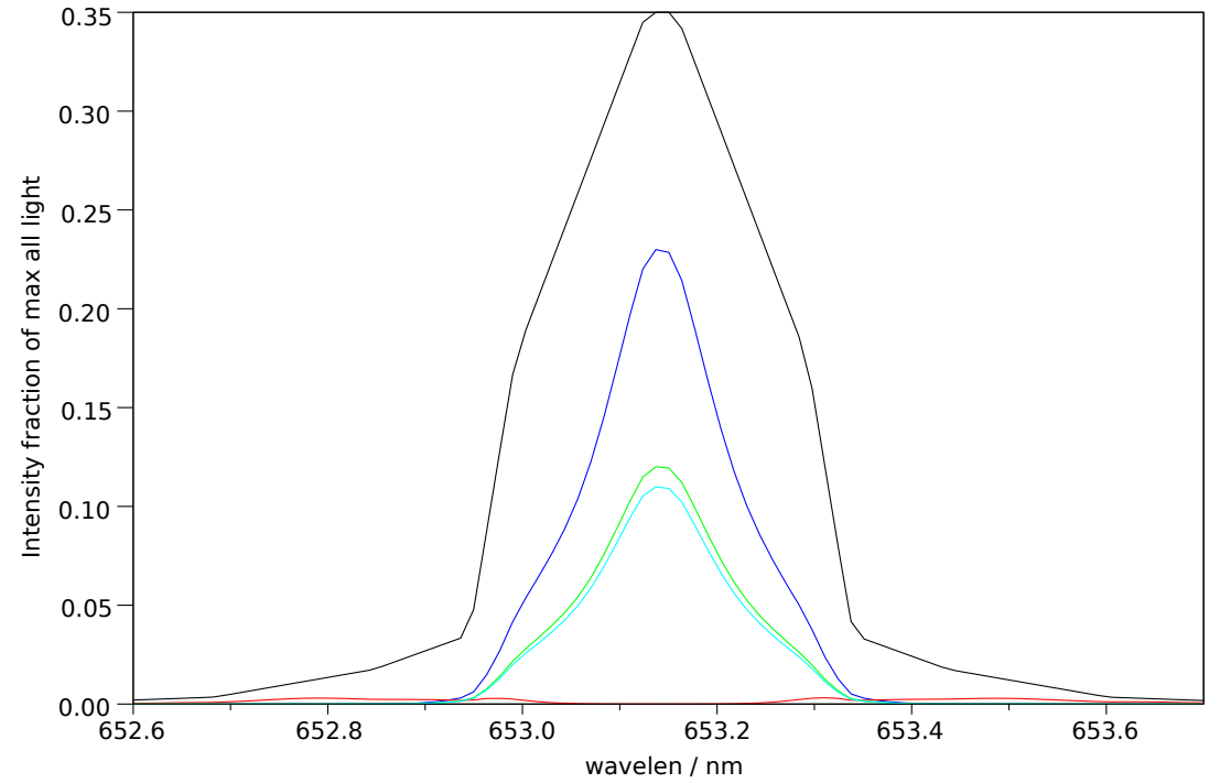
Filter 2: Makeup: Good= 66.1%, bad= 1.1%, unpol= 32.8% , good-unpol=33.3%. Total good transmitted= 25.6%
