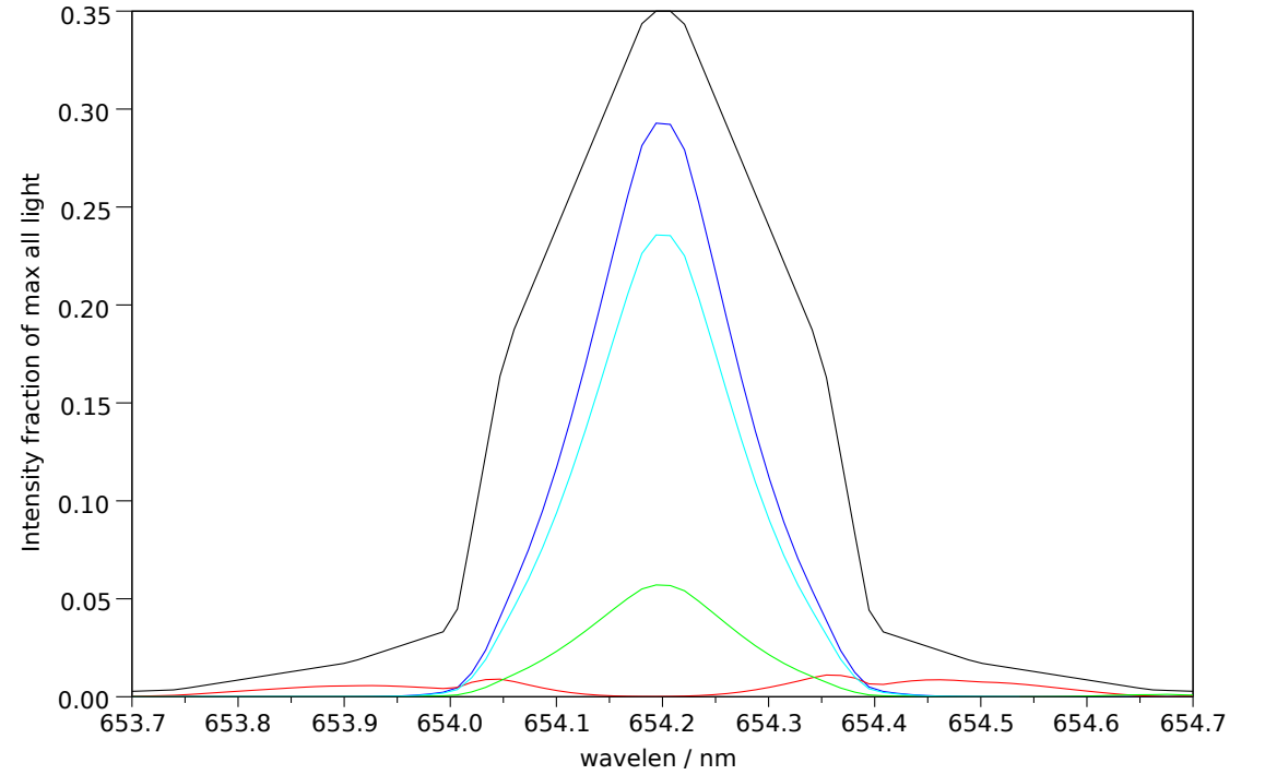
Filter 2: Makeup: Good= 78.3%, bad= 6.3%, unpol= 15.3% , good-unpol=63.0%. Total good transmitted= 26.6%
