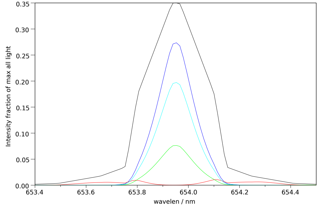
Filter 2: Makeup: Good= 73.6%, bad= 6.1%, unpol= 20.3% , good-unpol=53.3%. Total good transmitted= 26.9%
