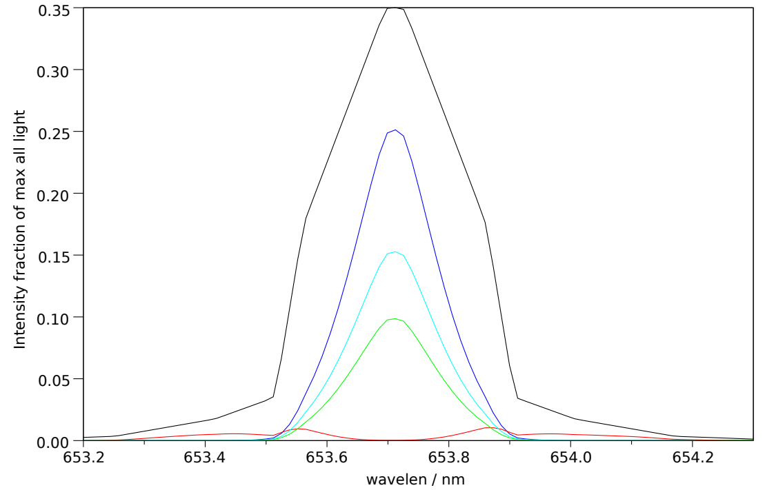
Filter 2: Makeup: Good= 68.2%, bad= 5.5%, unpol= 26.3% , good-unpol=41.8%. Total good transmitted= 27.1%
