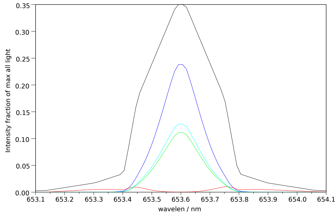
Filter 2: Makeup: Good= 65.0%, bad= 5.2%, unpol= 29.8% , good-unpol=35.1%. Total good transmitted= 27.2%
