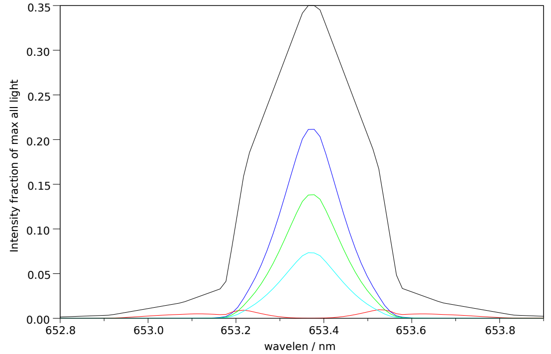
Filter 2: Makeup: Good= 58.3%, bad= 4.3%, unpol= 37.4% , good-unpol=21.0%. Total good transmitted= 27.4%
