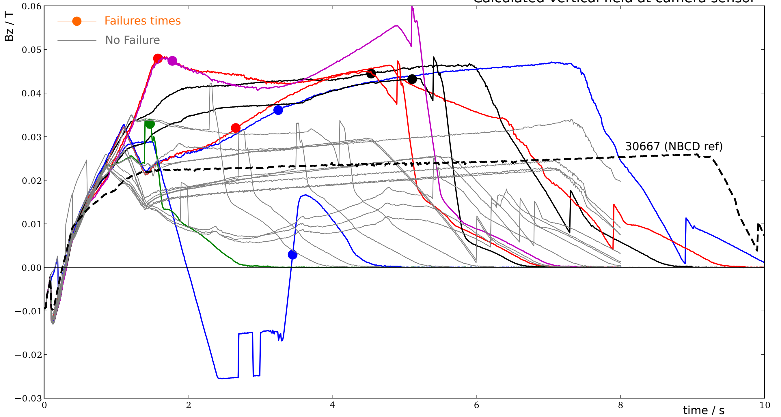
Calculated vertical field at camera sensor
